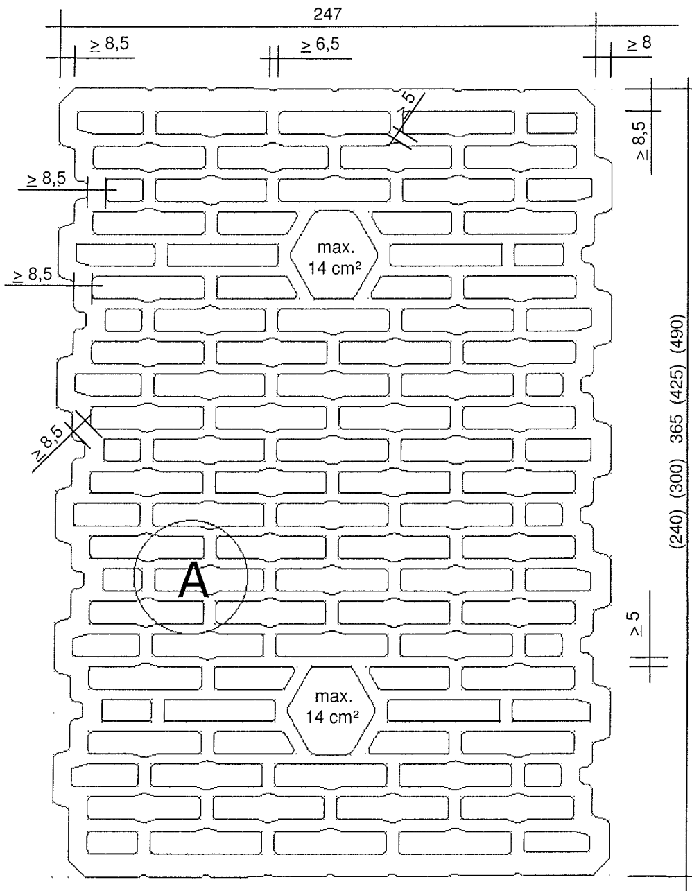
Detail A
